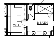
PRIMARY BATH ALTERNATIVE LAYOUT 2
